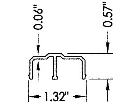
11 ROLLER TRACK
