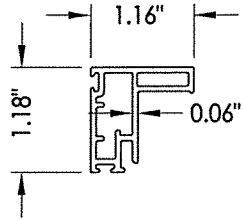
2 SASH STILE/RAIL
