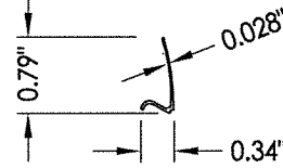
7 GLAZING BEAD
