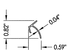
9 SCREEN CLIP
