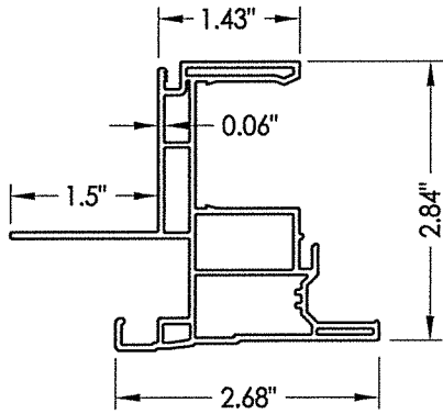
1 FRAME
