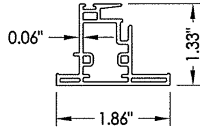
5 MEETING STILE
