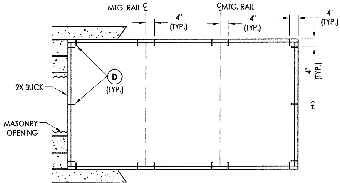
BUCK ANCHORING
